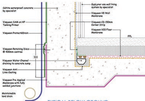
TYPICAL BELOW GROUND WALL/ FLOOR DETAIL : NEW CONCRETE (OPC)
