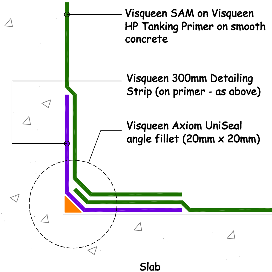
TYPICAL INTERNAL ANGLE FILLET DETAIL
