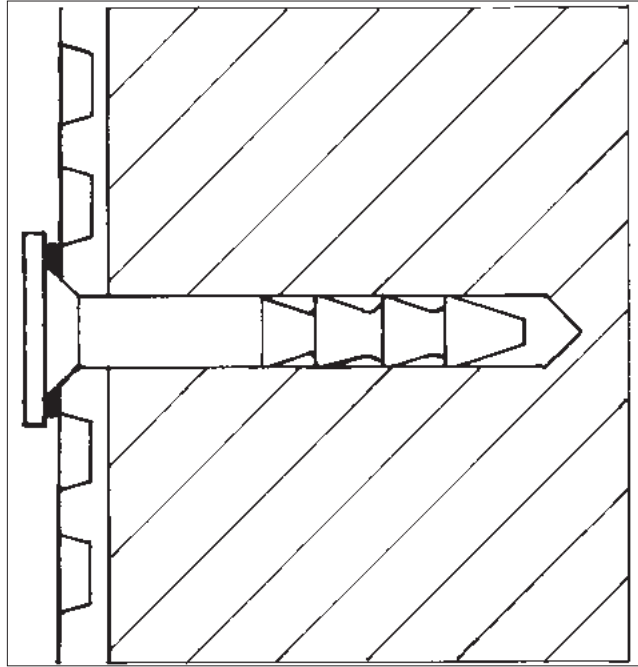
Figure 2 Visqueen Masonry Plug fixing detail
